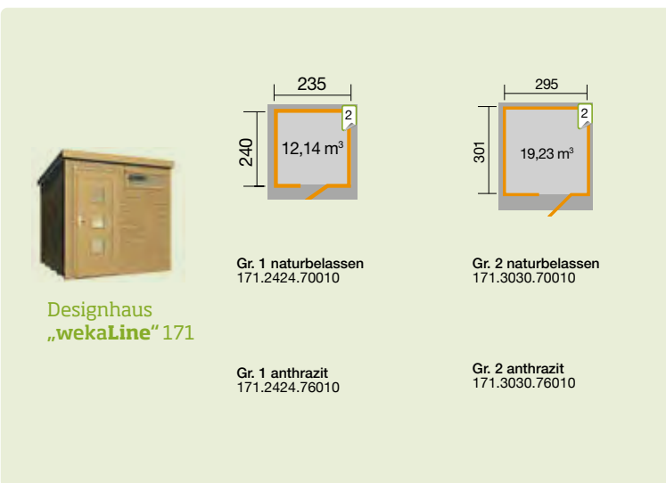
Designhaus wekaLine 171 Gr. 1 - 171.2424.76010
